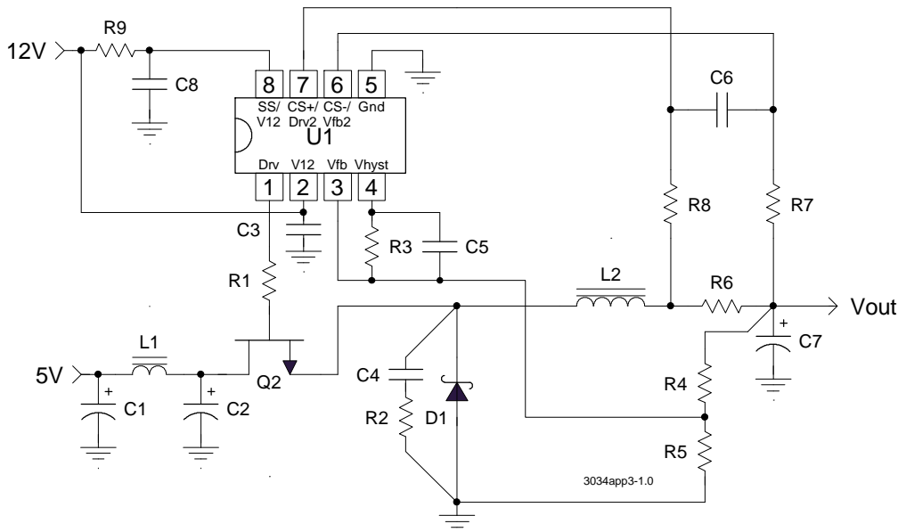
Figure4- The circuit in figure 4 is the application of the US3034 which is done using a dual layout with US3033 in a switching mode only. This circuit can be used to generate a low cost 5V to 3.3V for either Pentium application with AGP socket or in Pentium II applications where it is desirable to generate an accurate on board 3.3V supply.
