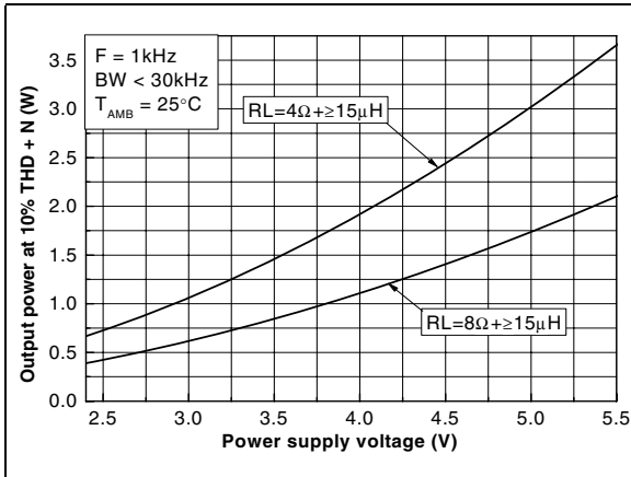
Figure 14. Output power vs. power supply voltage
