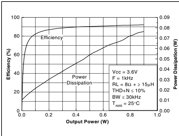
Figure 12. Efficiency vs. output power
