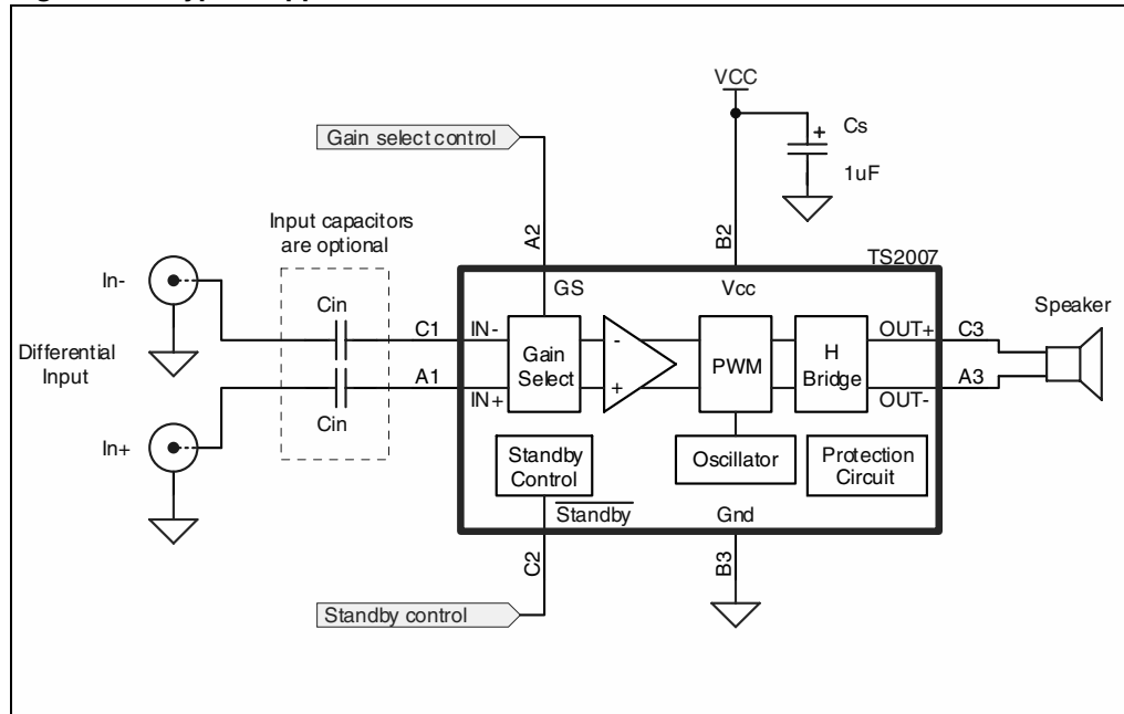
Figure 1. Typical application
