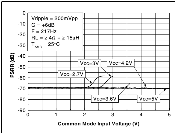
Figure 30. PSRR vs. common mode input voltage
