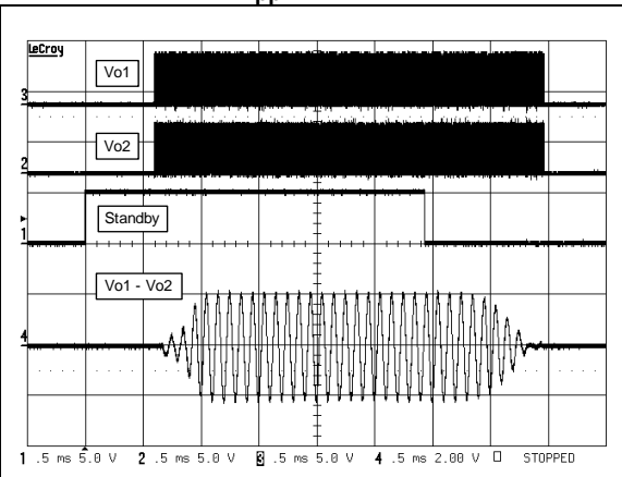
Figure 43. Startup and shutdown phase V_{CC}=5\text{ V} , G=12\text{ dB} , C_{in}=1\text{ }\mu\text{F} , V_{in}=1\text{ V}_{pp} , F=10\text{ kHz}
