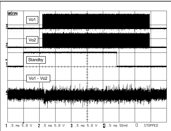
Figure 41. Startup and shutdown phase V_{CC}=5\text{ V} , G=6\text{ dB} , C_{in}=1\text{ }\mu\text{F} , inputs grounded
