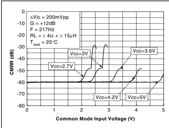
Figure 34. CMRR vs. common mode input voltage
