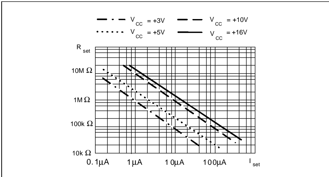
Figure 1 : R SET Connected to V CC - .
