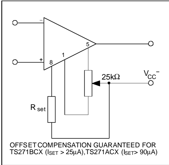
Figure 1 : R SET Connected to V CC - .
