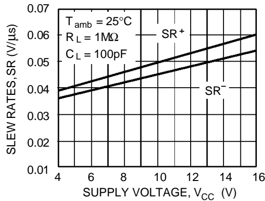
Figure 10 : Slew Rates versus Supply Voltage
