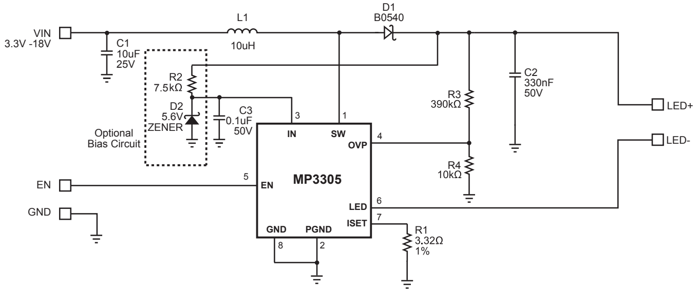
Figure 4 — Driving 27 WLEDs (9 WLEDs in Series and 3 Strings Paralleled) with 3.3V-18V Input Voltage
