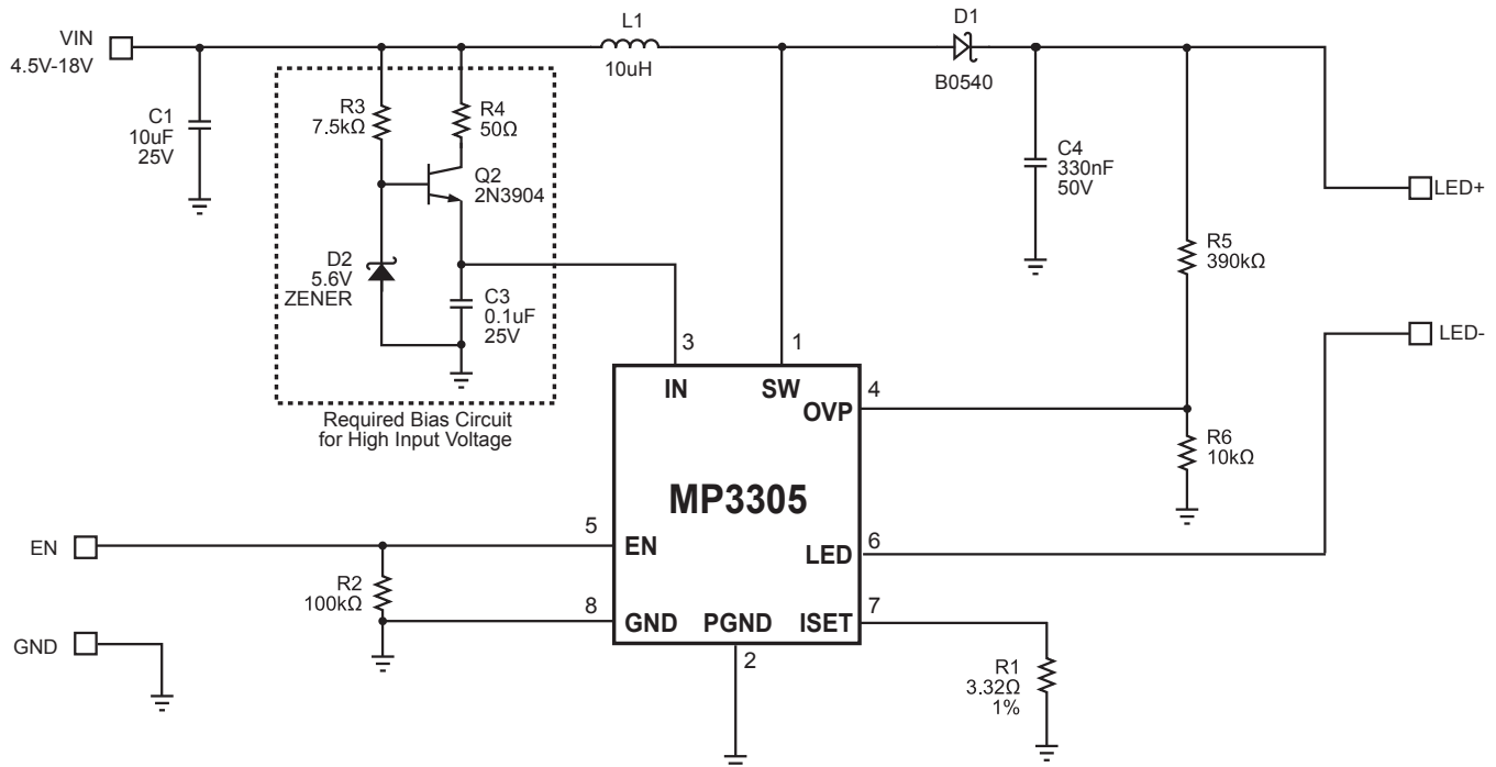
Figure 5 — Wide Input Voltage Step-up Converter for 27 WLEDs (9 WLEDs in Series and 3 Strings Paralleled)
