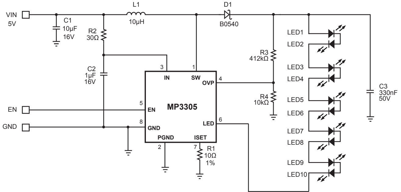
Figure 6 — Driving 10 WLEDs in Series with 5V Input Voltage
