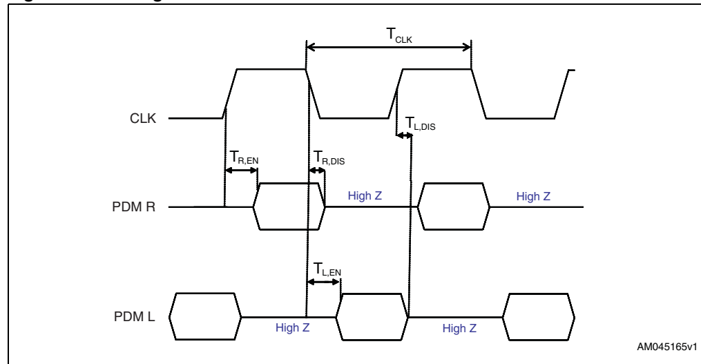
Figure 2. Timing waveforms
