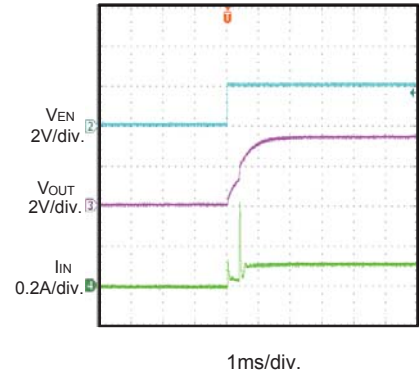
Inrush Current
