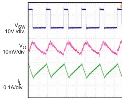
400ns/div
