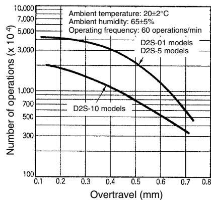
Mechanical Durability (Pin Plunger Models)
