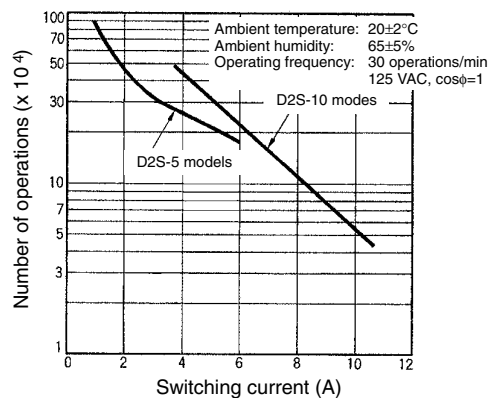
Electrical Durability (Pin Plunger Models)
