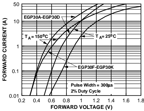
Forward Characteristics
