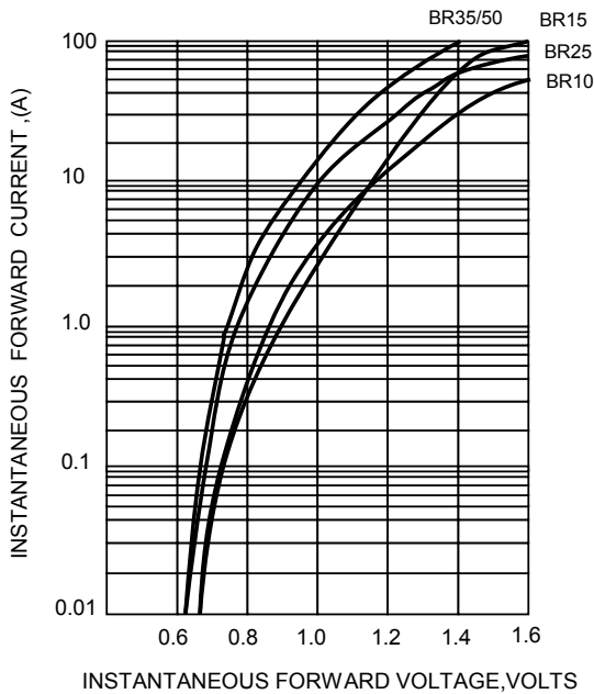
FIG.3-TYPICAL FORWARD CHARACTERISTICS
