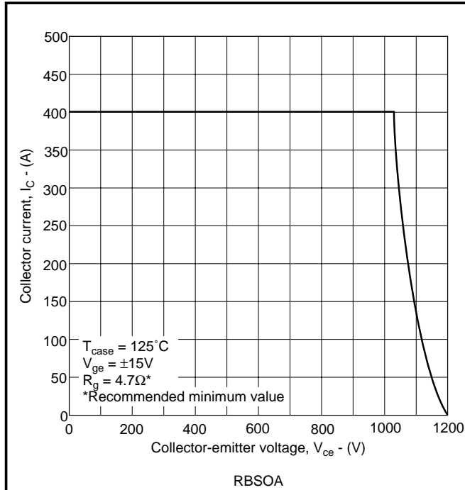
Fig. 11 Forward bias safe operating area
