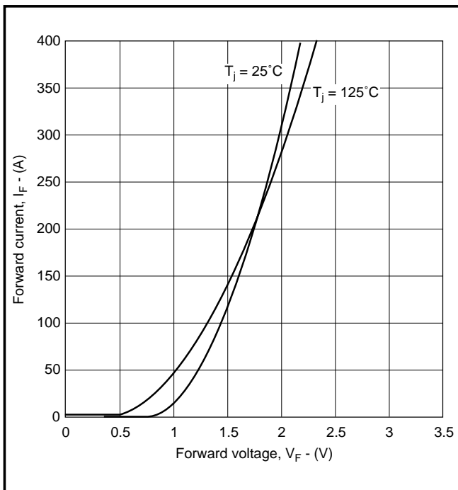
Fig. 9 Freewheel diode typical forward characteristics
