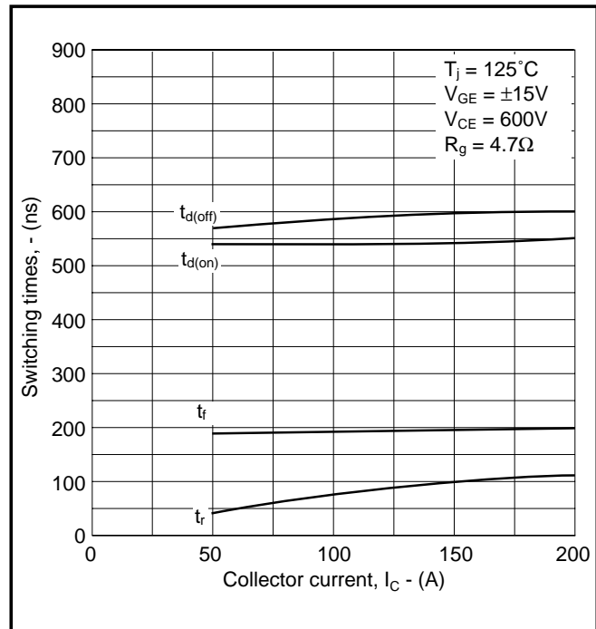
Fig. 8 Typical switching characteristics
