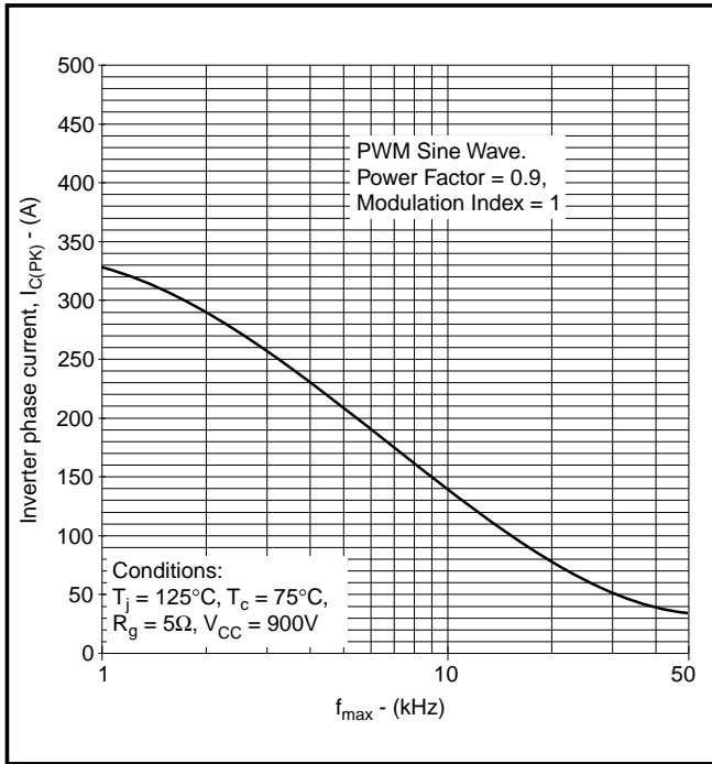
Fig. 12 3 Phase inverter operating frequency
