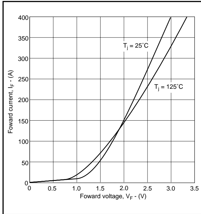
Fig. 11 Diode typical forward characteristics
