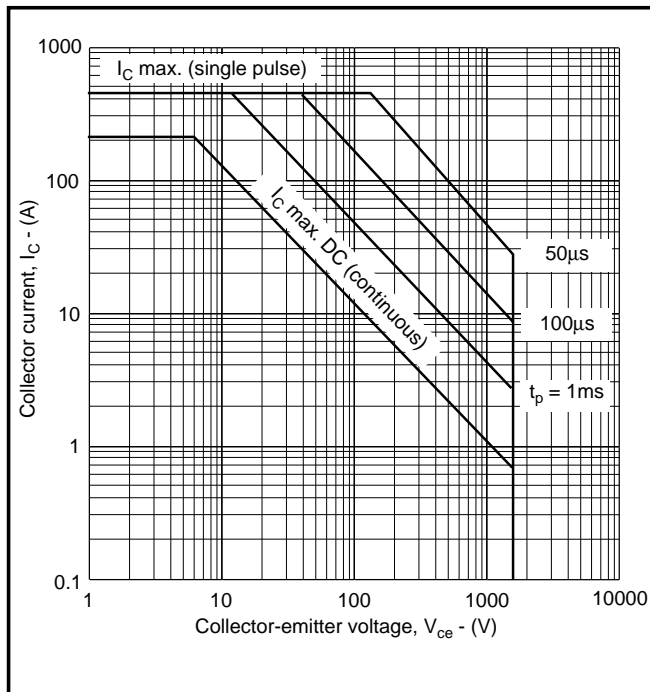
Fig. 13 Forward bias safe operating area
