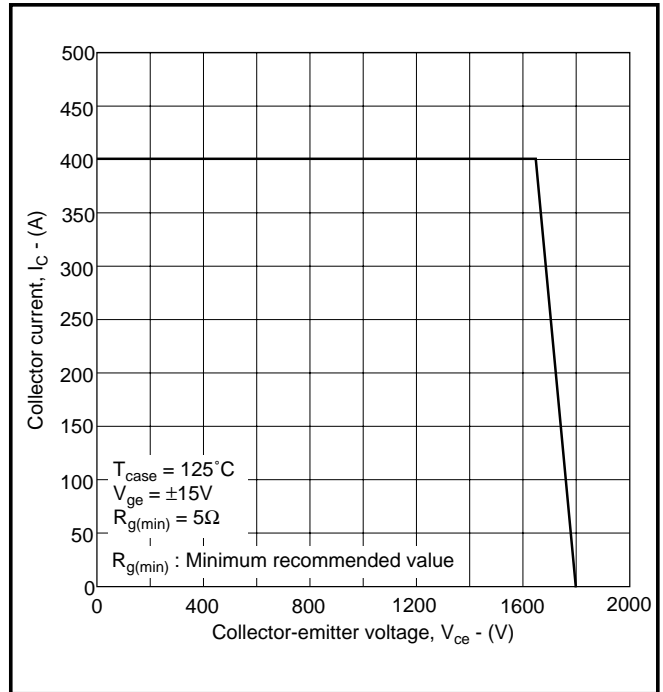
Fig. 12 Reverse bias safe operating area
