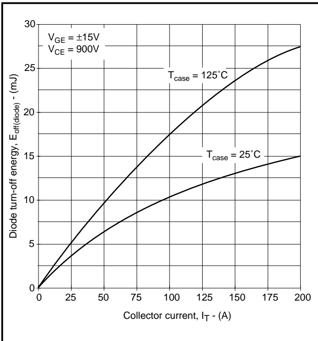
Fig. 9 Typical diode turn-off energy vs collector current
