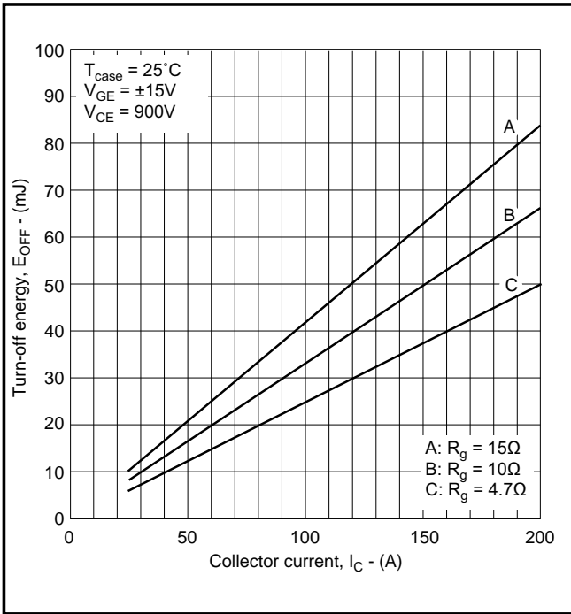
Fig. 7 Typical turn-off energy vs collector current
