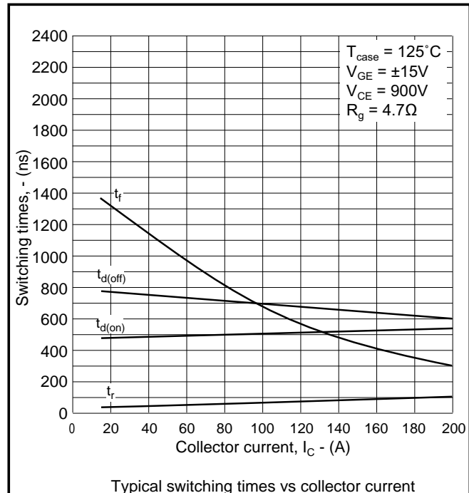
Fig. 10 Typical switching characteristics vs collector current
