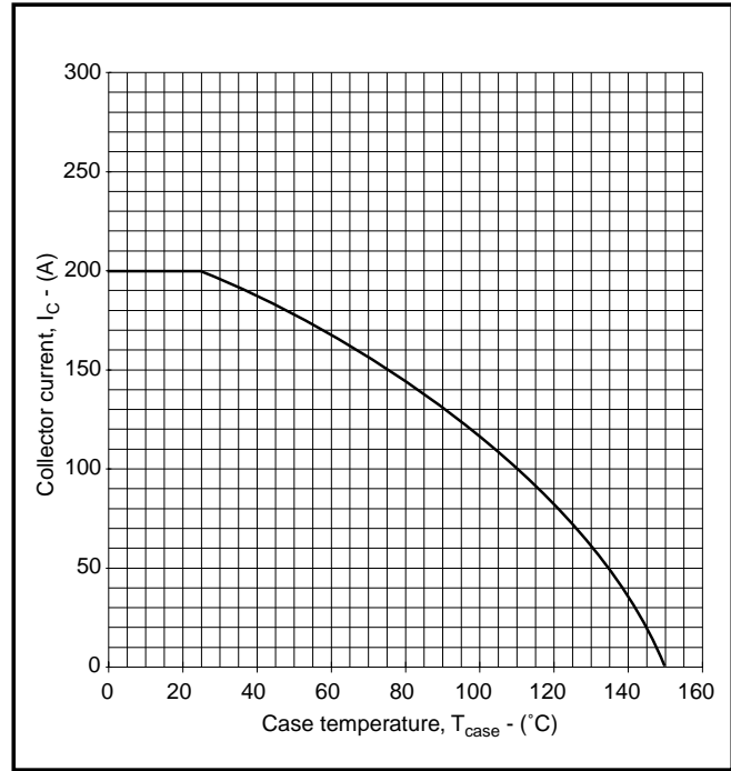
Fig. 13 DC current rating vs case temperature
