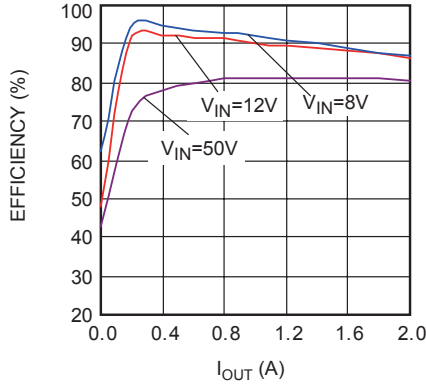
Efficiency vs. Load Current V_{OUT}=5\text{V}
