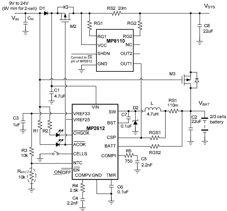
Figure 2—Switching Charger with Power Path Management (1)
