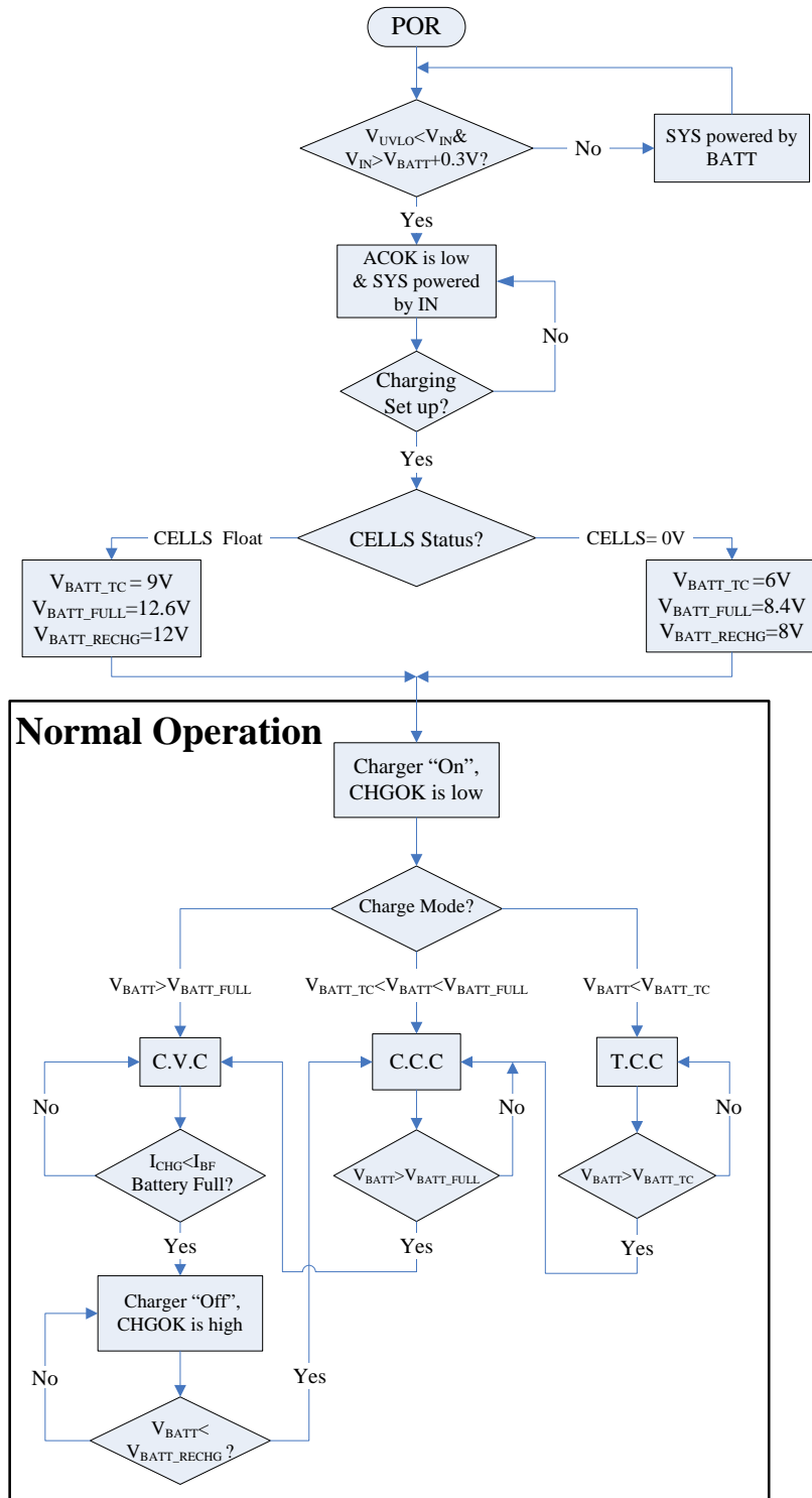
Figure 6— Normal Charging Operation Flow Chart
