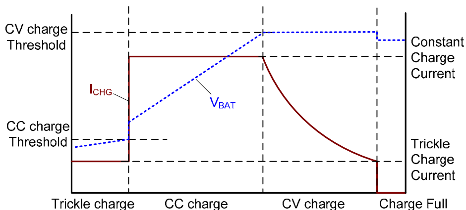
Figure 4—Li-Ion Battery Charge Profile
