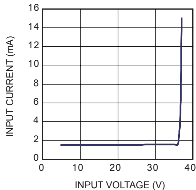
Breakdown Voltage
