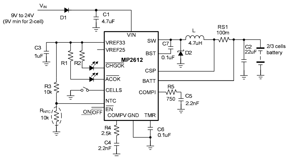
Figure 1—Standalone Switching Charger
