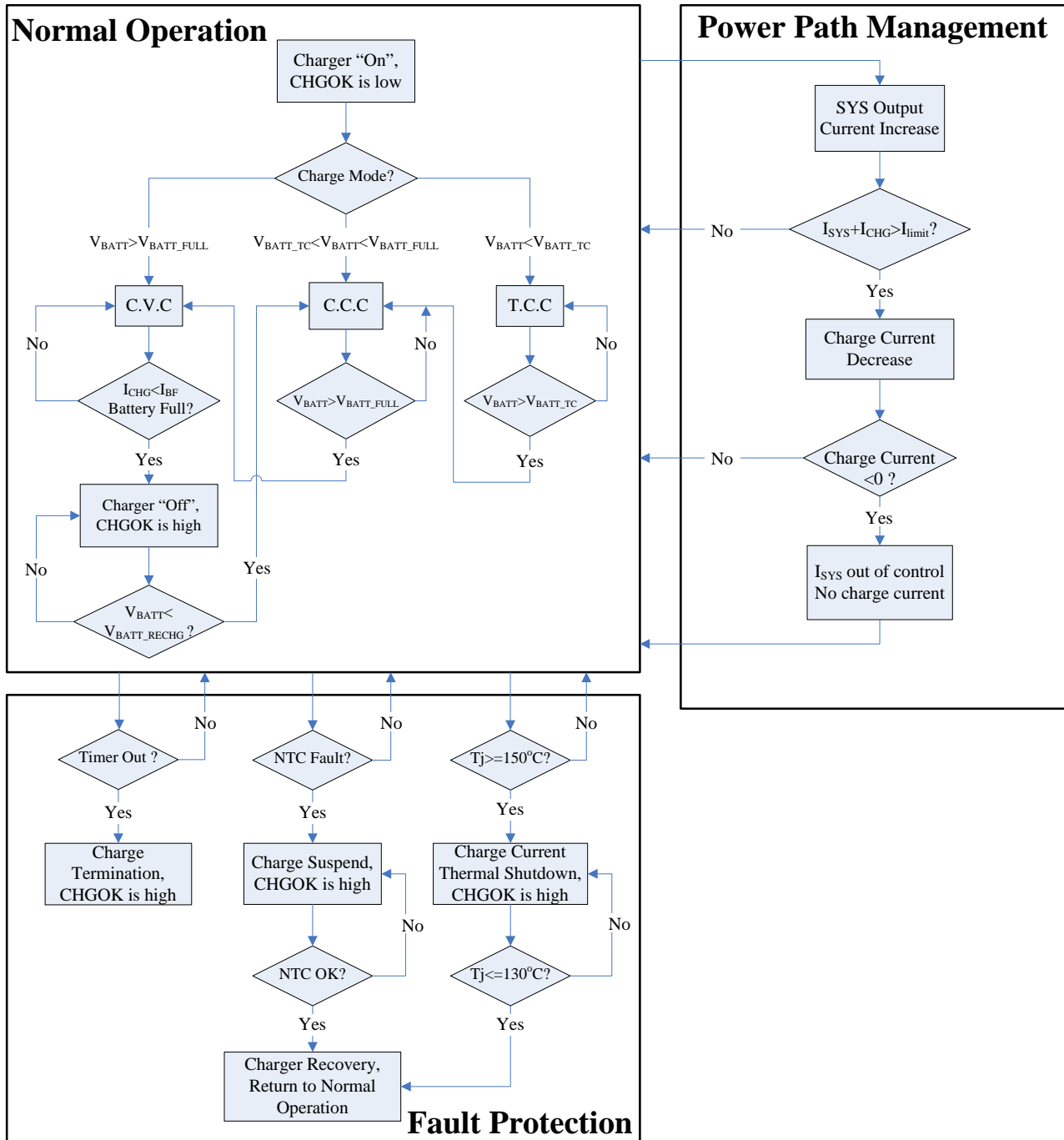
Figure 7— Power Path Management Operation and Fault Protection Flow Chart
