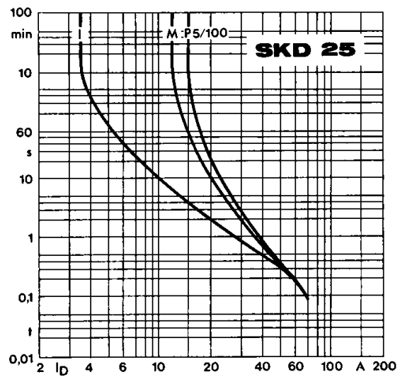
Fig. 6 b Rated overload current vs. time
