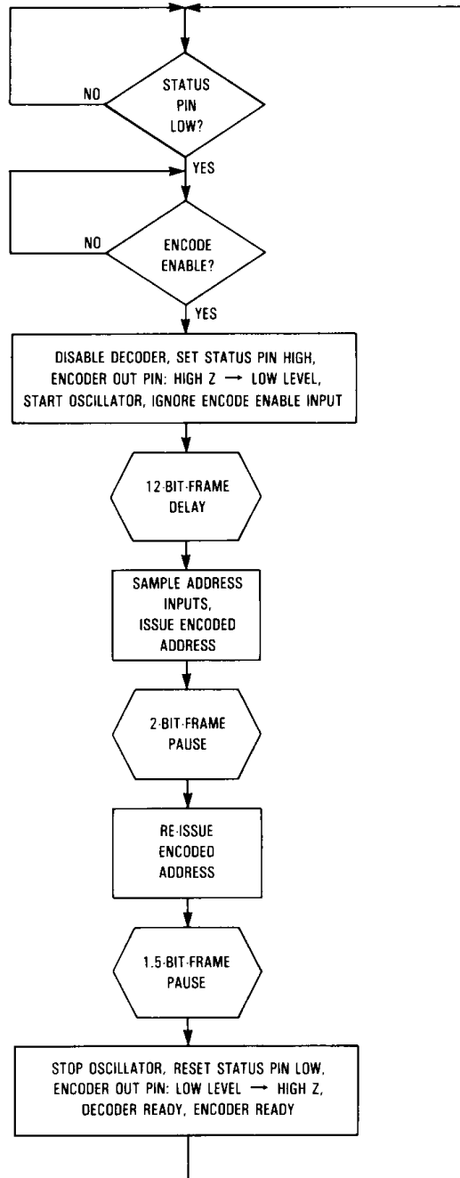
Figure 8. Encoder Flowchart
