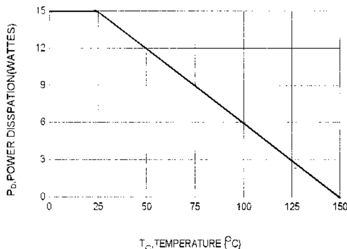
FIGURE -1 POWER DERATING
