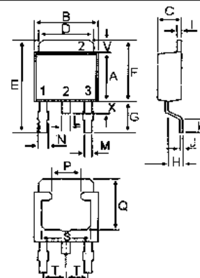
TO-252AA (DPAK)
