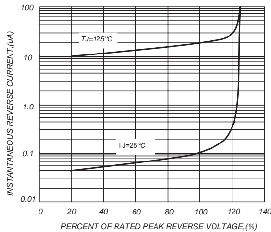
FIG.5-TYPICAL REVERSE CHARACTERISTICS
