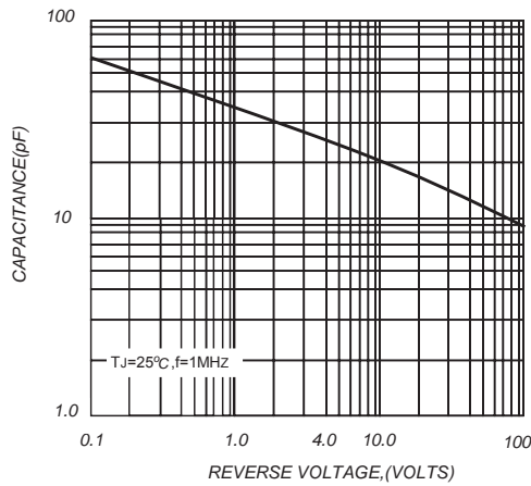
FIG.3-TYPICAL JUNCTION CAPACITANCE
