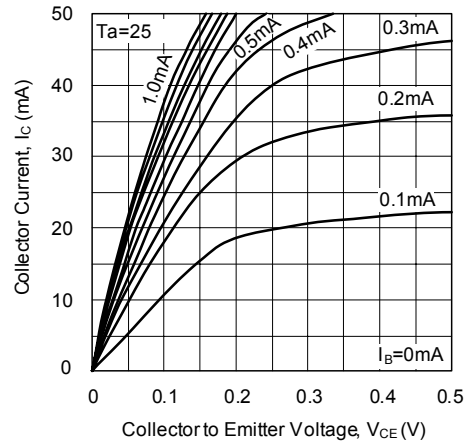
Grounded Emitter Output Characteristics ( )
