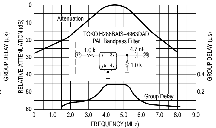
Figure 6b. Group Delay and Magnitude Response of the TOKO Bandpass Filter Intended for PAL Applications
