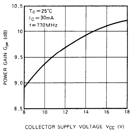
POWER GAIN VS. COLLECTOR SUPPLY VOLTAGE
