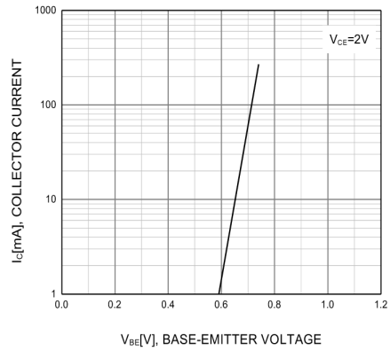
Figure 4. Base-Emitter On Voltage
