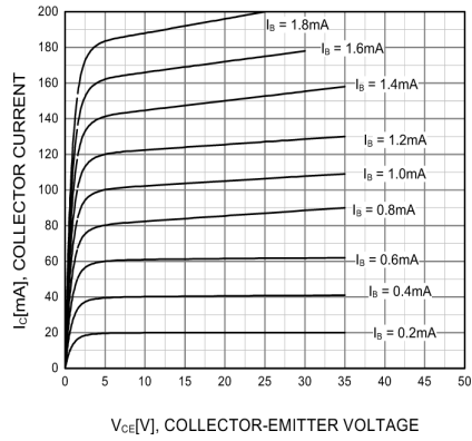
Figure 1. Static Characteristic
