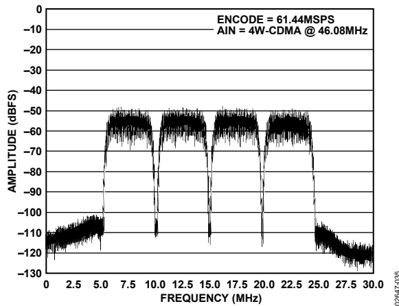
Figure 29. Four W-CDMA Carriers @ 46.08 MHz, Encode = 61.44 MS/SPS
