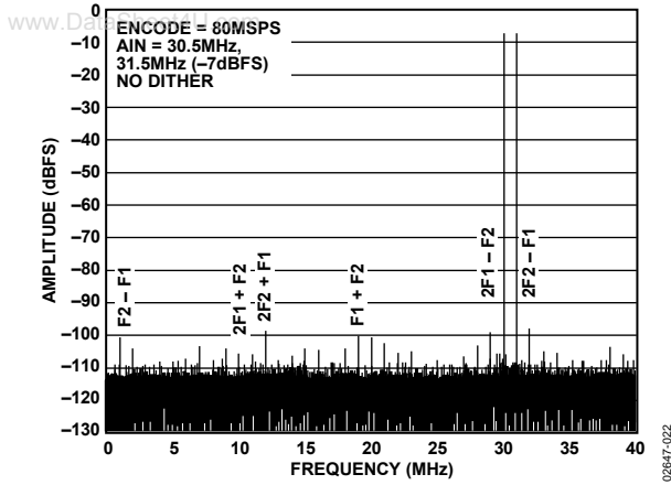
Figure 16. Two-Tone SFDR @ 30.5 MHz and 31.5 MHz
