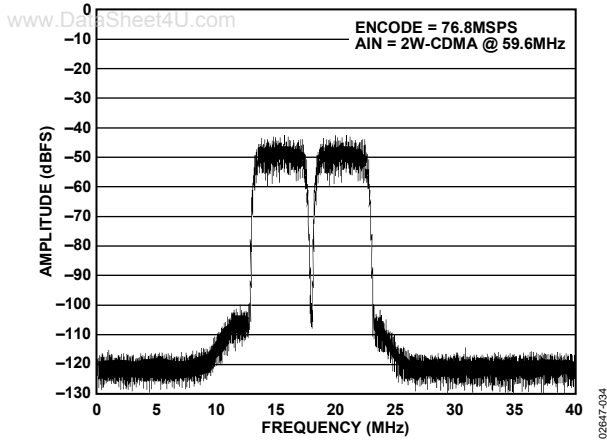
Figure 28. Two W-CDMA Carriers @ 59.6 MHz, Encode = 76.8 MS/SPS
