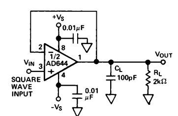
Figure 21c. Unity Gain Follower
