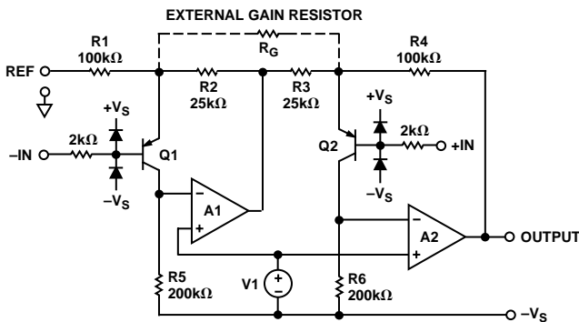
Figure 32. Simplified Schematic
