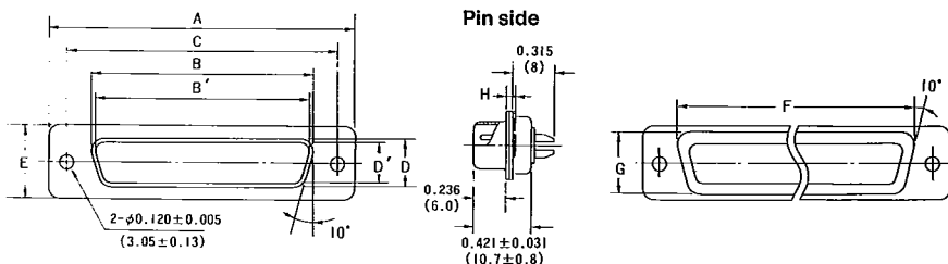
Dimensions when mated
