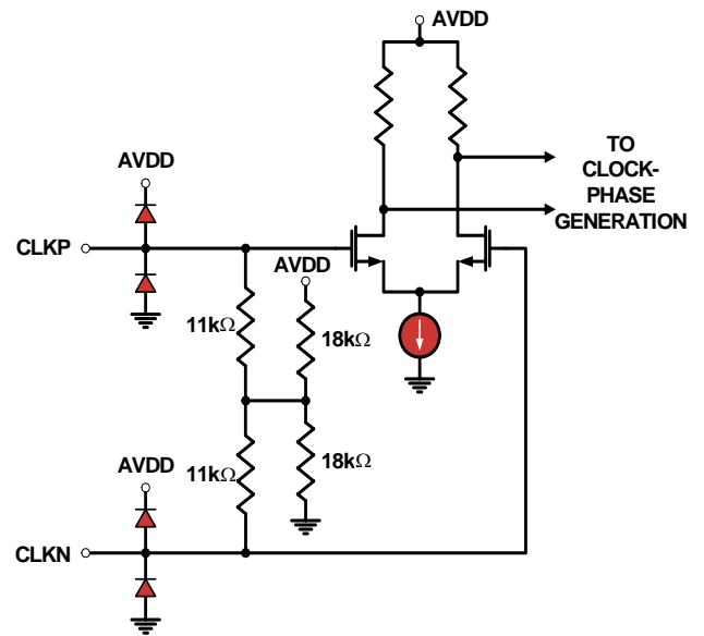
FIGURE 48. CLOCK INPUTS
