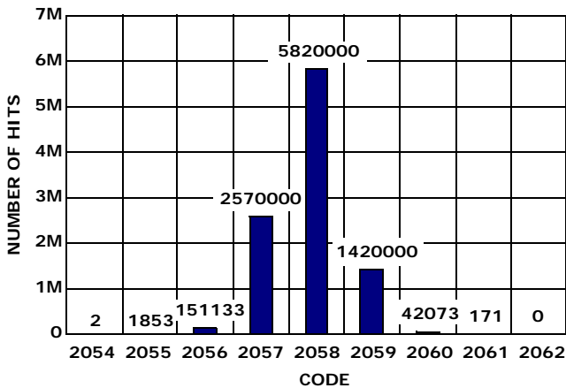
FIGURE 14. NOISE HISTOGRAM
