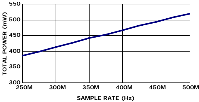
FIGURE 10. POWER vs fSAMPLE IN 3mA LVDS MODE
