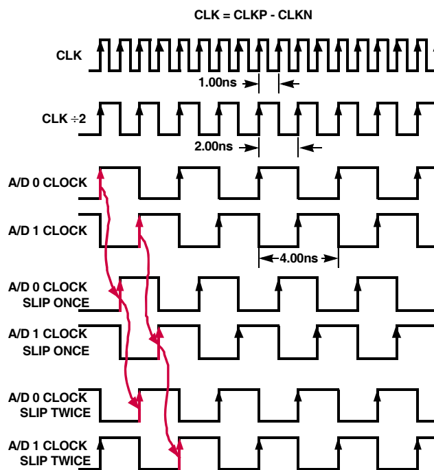
FIGURE 45. PHASE SLIP: CLK/2 MODE, f_{\text{CLOCK}} = 1000\text{MHz}
