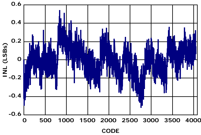
FIGURE 12. INTEGRAL NONLINEARITY
