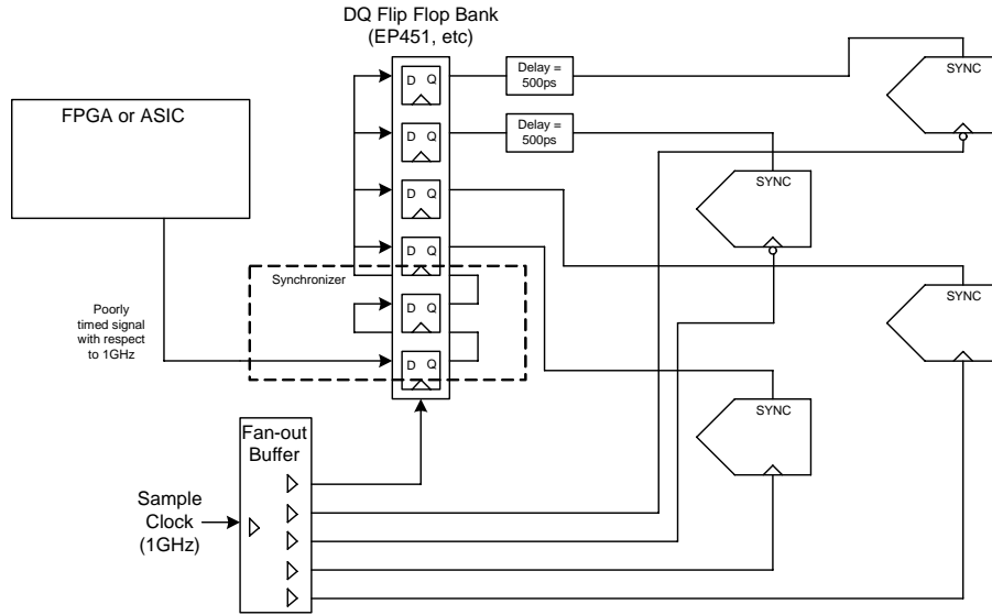
FIGURE 38. SYNCHRONIZATION SCHEME
