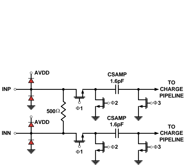
FIGURE 47. ANALOG INPUTS
