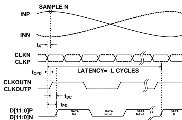
FIGURE 3. CMOS TIMING DIAGRAM
