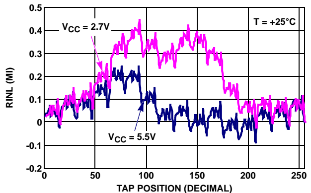
FIGURE 12. RINL vs TAP POSITION IN RHEOSTAT MODE FOR 50kΩ (U)
