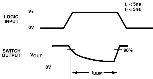
FIGURE 3A. t_{BDM} MEASUREMENT POINTS
