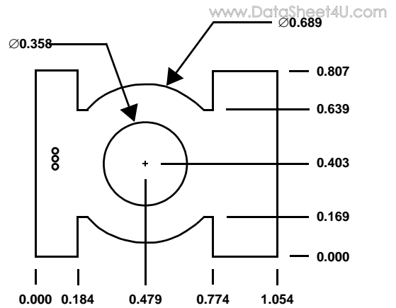
FIGURE 7G. PWB DIMENSIONS
