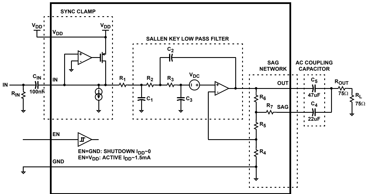
FIGURE 24. BLOCK DIAGRAM
