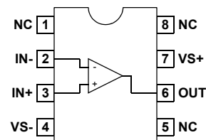
ISL55001 (8 LD SO) TOP VIEW
