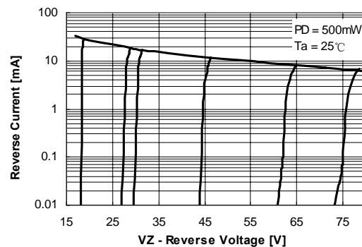
Figure 6. Reverse Current vs. Reverse Voltage
