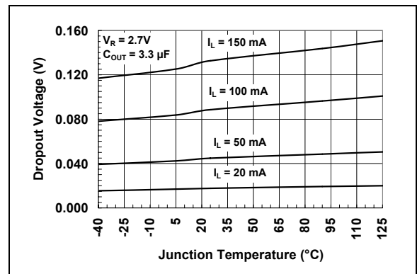
FIGURE 2-12: Dropout Voltage vs. Junction Temperature.
