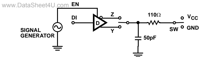
FIGURE 2. DRIVER PROPAGATION DELAY AND DIFFERENTIAL TRANSITION TIMES
