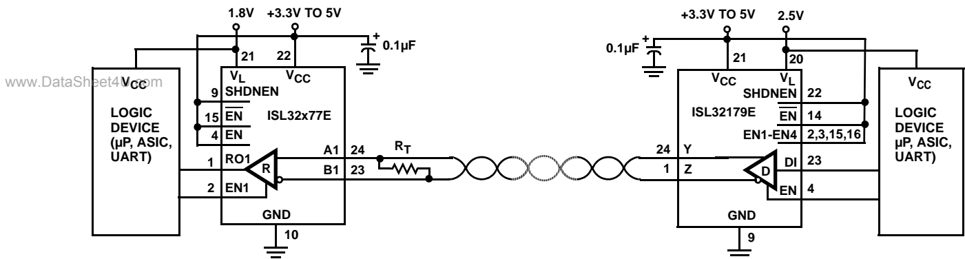
NETWORK WITH V L PIN FOR INTERFACING TO LOWER VOLTAGE LOGIC DEVICES
