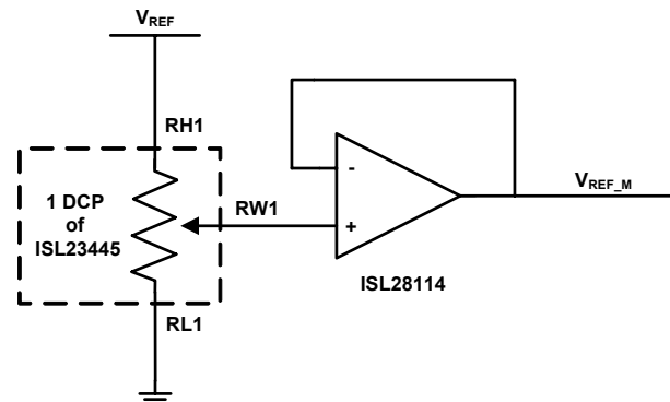
FIGURE 2. V_{REF} ADJUSTMENT
