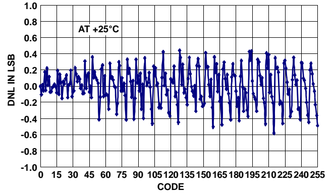
FIGURE 10. DNL, V_{REF} AND TEMP SLOPE DAC
