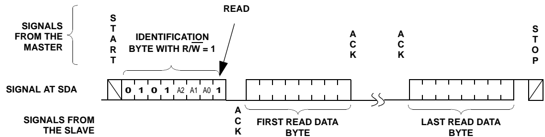
FIGURE 17. ADDRESS READ SEQUENCE
