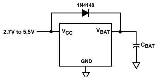
FIGURE 20. SUPERCAPACITOR CHARGING CIRCUIT
