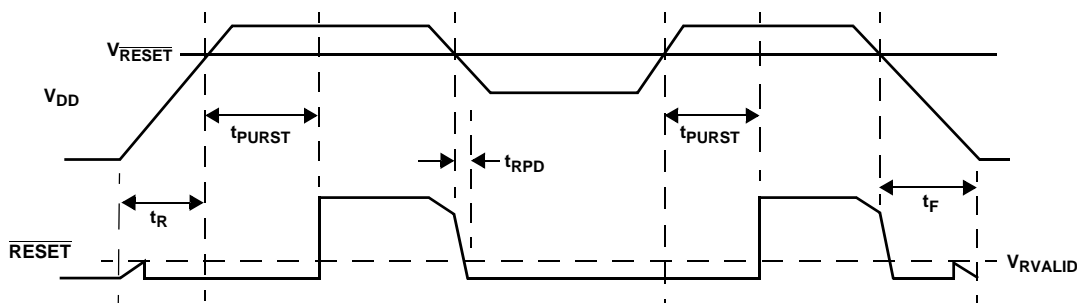
FIGURE 4. RESET TIMING
