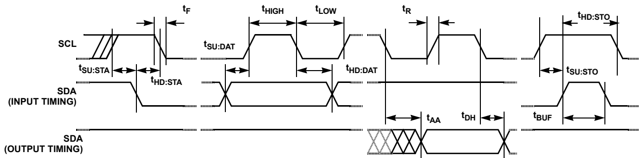
FIGURE 1. BUS TIMING
