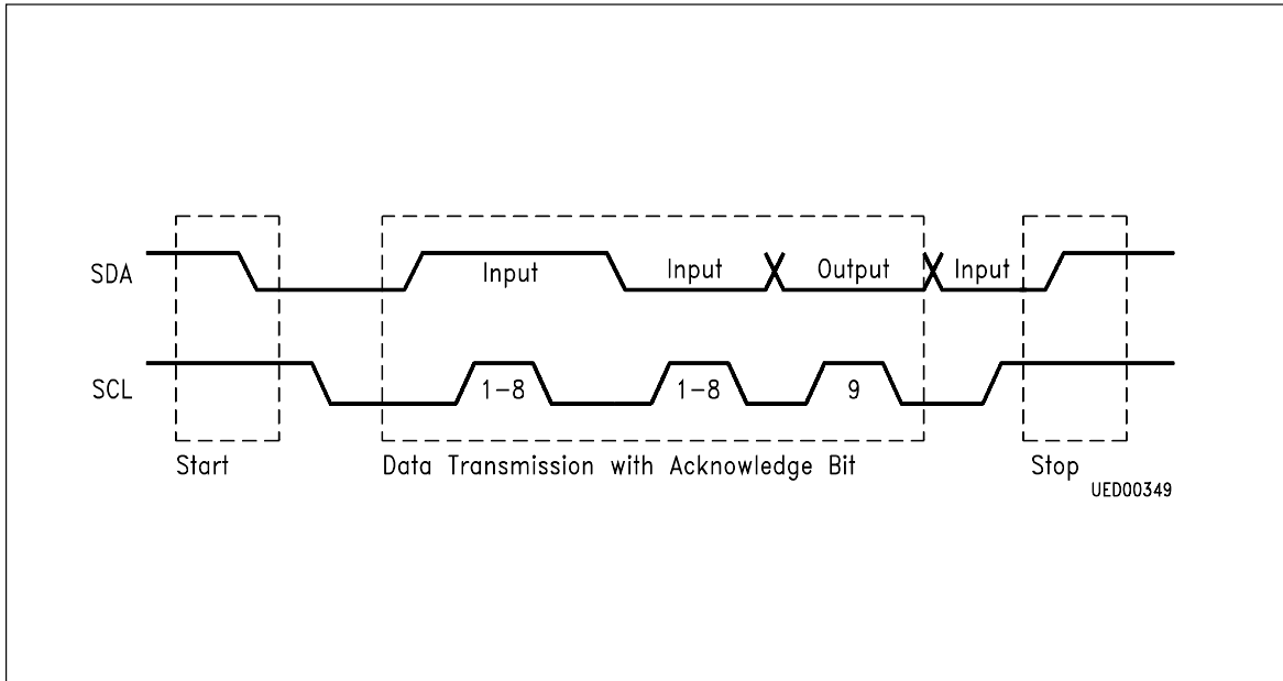
Figure 1 Operational States of the I 2 C Bus
