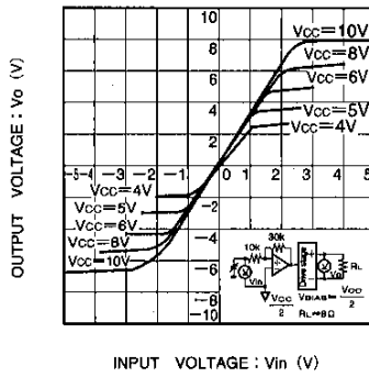
Fig. 6 Driver I/O characteristics (power supply variation)
