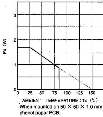
Fig. 5 Thermal derating curve
