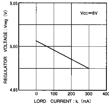
Fig. 12 Load current vs. regulator voltage
