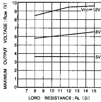
Fig. 9 Load resistance vs. maximum output amplitude
