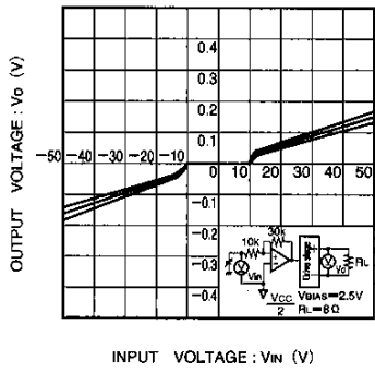
Fig. 8 Dead zone I/O characteristics
