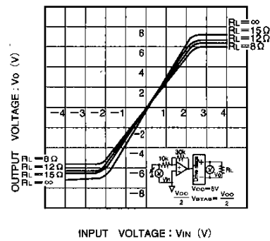
Fig. 7 Driver I/O characteristics (load variation)
