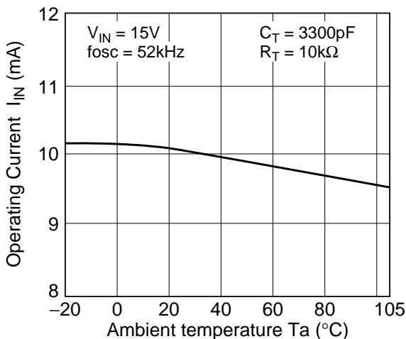
Operating Current vs. Ambient Temperature
