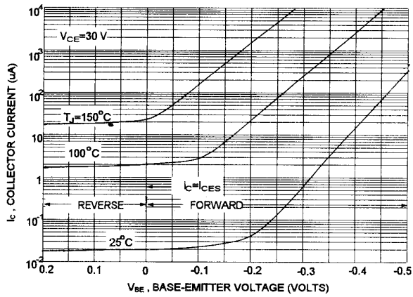
VBE, BASE-EMITTER VOLTAGE (VOLTS)
