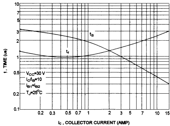
TURN-OFF TIME
