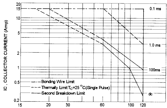
VCE, COLLECTOR EMITTER VOLTAGE (VOLTS) MJ2955A, MJ15016
