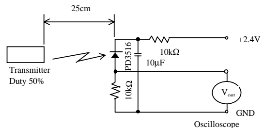
Fig 2. Standard Transmitter Measurement circuit
