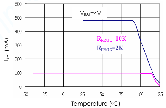
Charge Current vs Ambient Temperature
