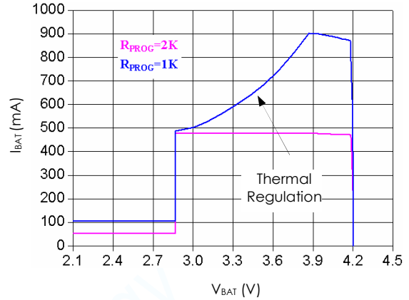
Charge Current vs Battery Voltage
