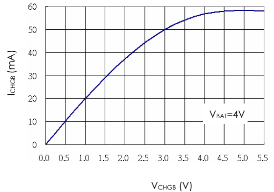
CHGB Pin I-V Curve (Strong Pull-Down State)
