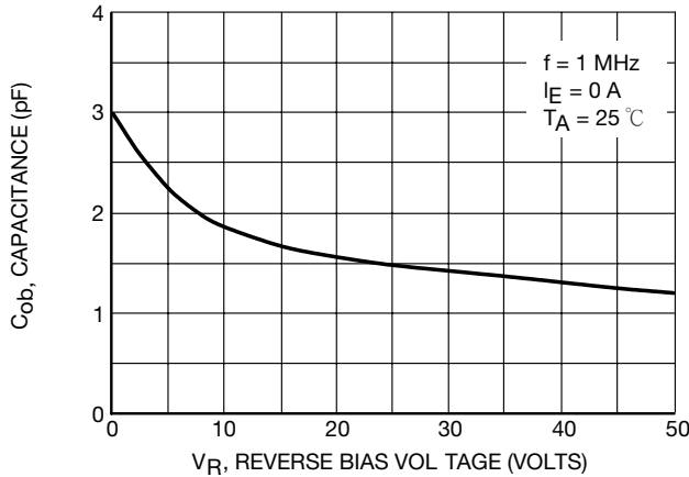
Figure 9. Output Capacitance
