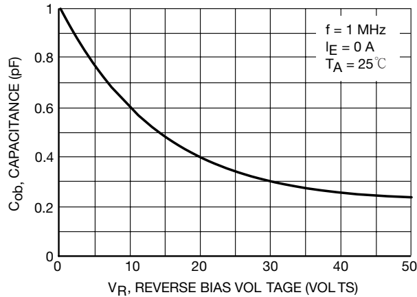
Figure 14. Output Capacitance
