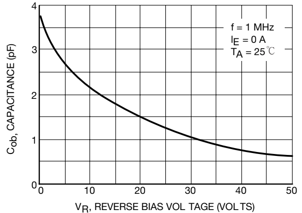
Figure 4. Output Capacitance
