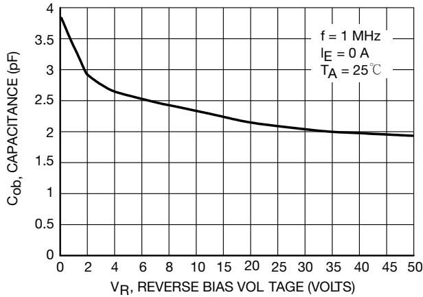
Figure 19. Output Capacitance
