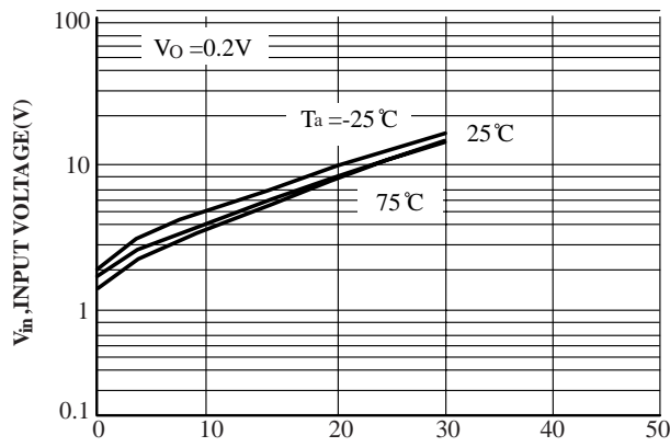
IC, COLLECTOR CURRENT(mA) FIG.12 Input Voltage vs. Output Current
