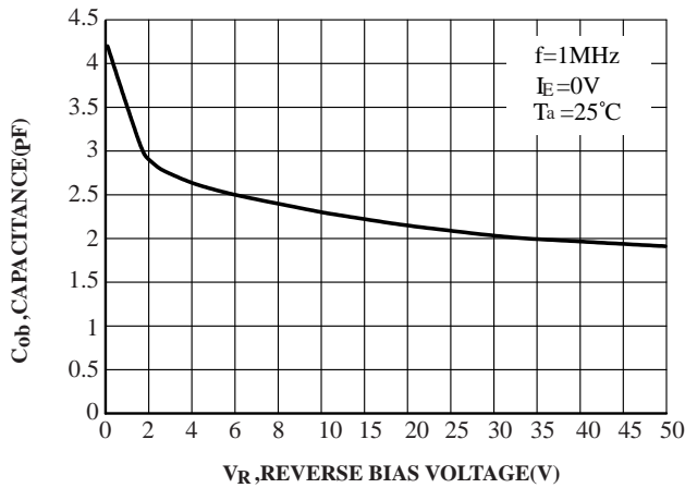
FIG.20 Output Capacitance
