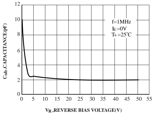
FIG.25 Output Capacitance
