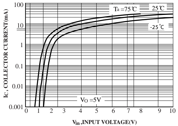
FIG.16 Output Current vs. Input Voltage
