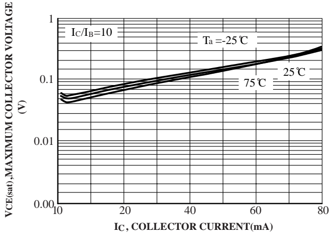
FIG.18 V_{CE(sat)} vs. I_C
