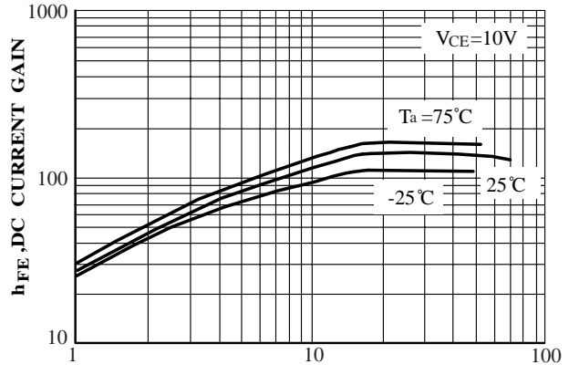
IC, COLLECTOR CURRENT(mA) FIG.9 DC Current Gain
