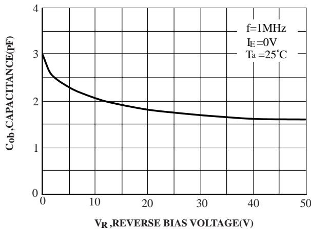
FIG.5 Output Capacitance
