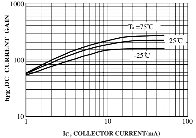
FIG.14 DC Current Gain
