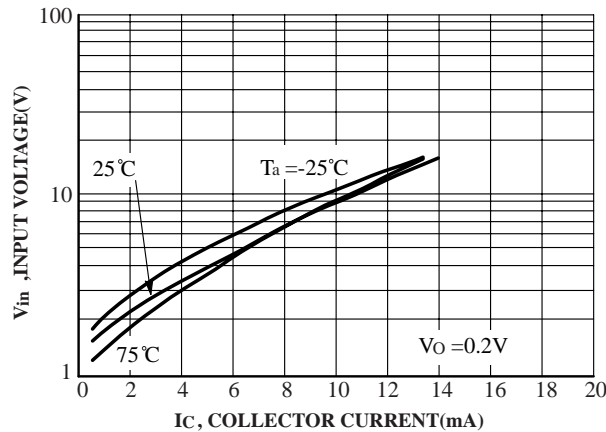
FIG.32 Input Voltage Versus Output Current
