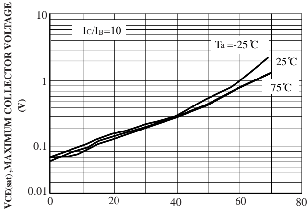
IC, COLLECTOR CURRENT(mA) FIG.8 VCE(sat) vs. IC
