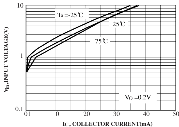
FIG.22 Input Voltage vs. Output Current
