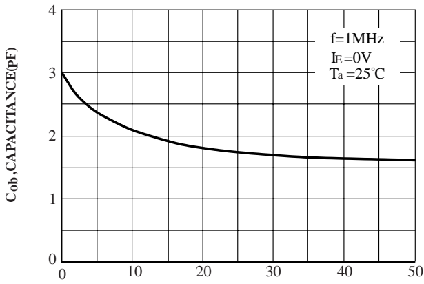
VR, REVERSE BIAS VOLTAGE(V) FIG.10 Output Capacitance
