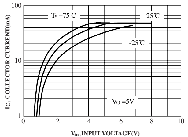
FIG.21 Output Current vs. Input Voltage
