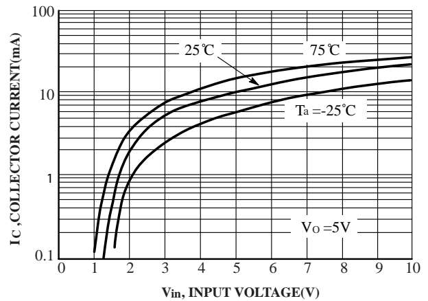
FIG.31 Output Current Versus Input Voltage
