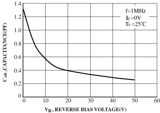
FIG.35 Output Capacitance
