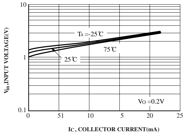
FIG.27 Input Voltage vs. Output Current
