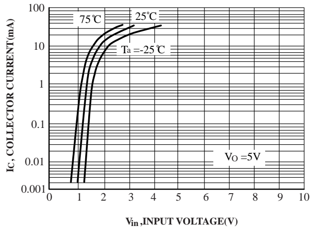
FIG.6 Output Current vs. Input Voltage
