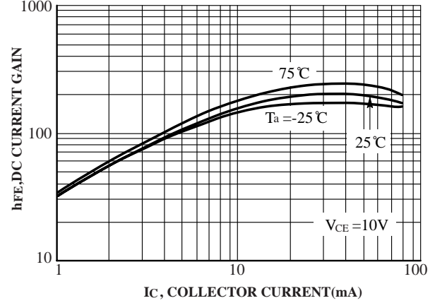
FIG.34 DC Current Gain
