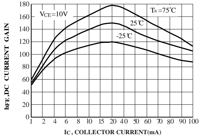
FIG.19 DC Current Gain
