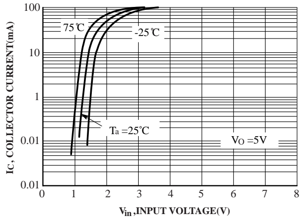
FIG.26 Output Current vs. Input Voltage
