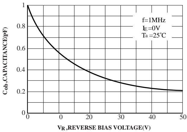
FIG.15 Output Capacitance
