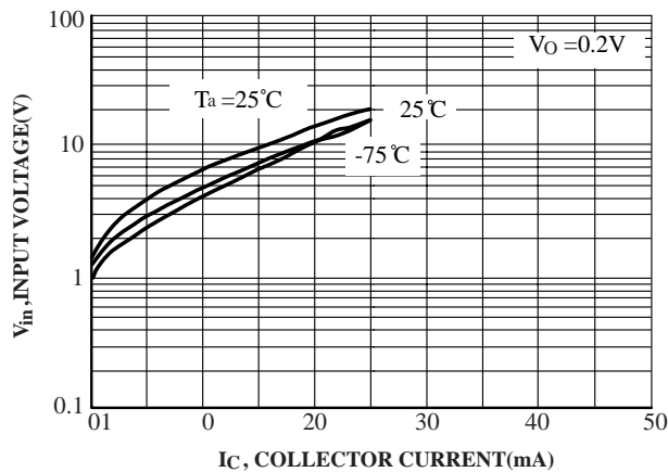
FIG.17 Input Voltage vs. Output Current
