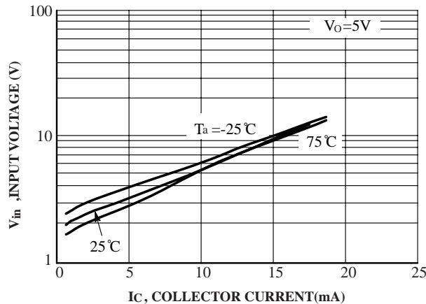
FIG.37 Input Voltage Versus Output Current
