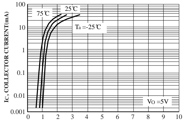
IC, COLLECTOR CURRENT (mA) FIG.11 Output Current vs. Input Voltage
