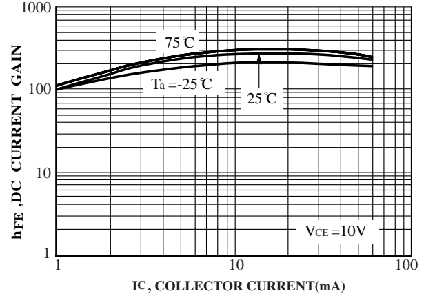
FIG.29 DC Current Gain
