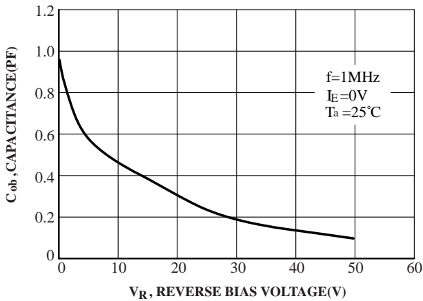
FIG.30 Output Capacitance
