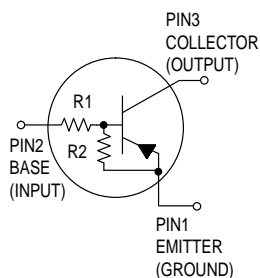
CASE 318D-03, STYLE 1 (SC-59)
