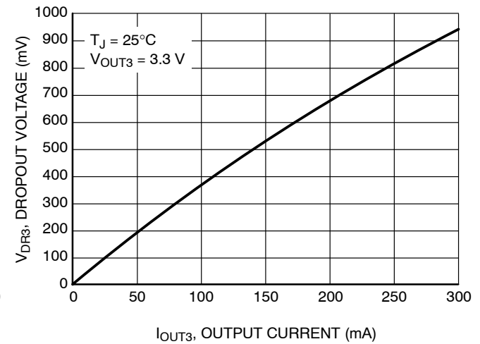
Figure 16. Dropout LDO3 vs Output Current
