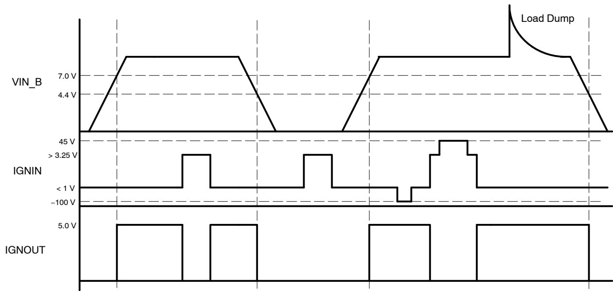
Figure 5. IGNOU Timing Diagram
