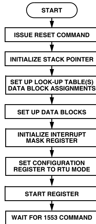
FIGURE 19 – RTU INITIALIZATION
