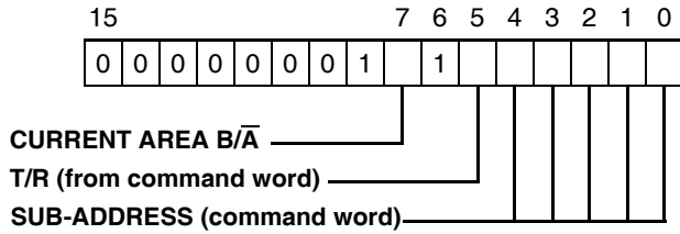
FIGURE 20 – RTU LOOK-UP ADDRESS
