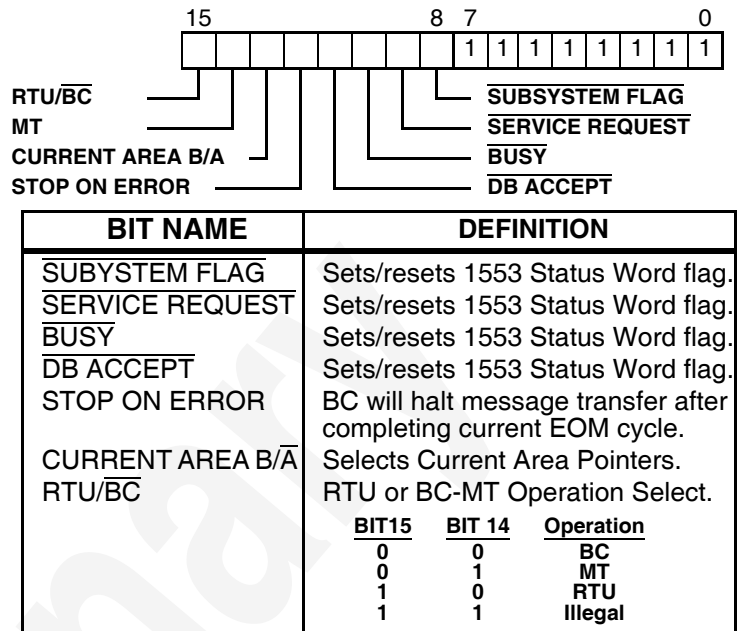
FIGURE 11 – CONFIGURATION REGISTER
