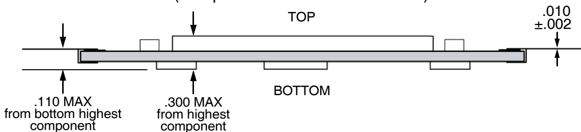
FLAT PCB SIDE VIEW (Components on both sides of PCB)
