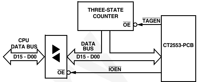
FIGURE 15 – BC/RT TAGGING (OPTIONAL)
